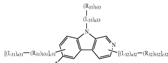
Formula 2F(1)
