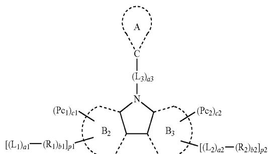
Formula 1C
