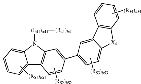
Formula 41-7
