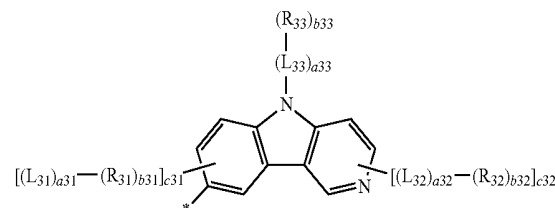
Formula 2F(2)
