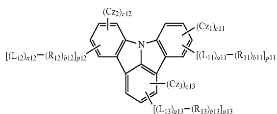
Formula 2A
