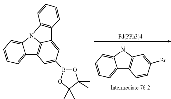
Intermediate 76-3
