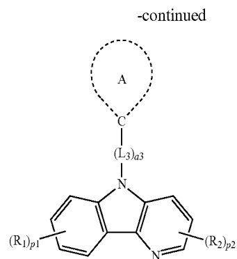
Formula 1B(5)
