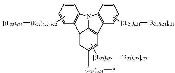
Formula 2E(1)
