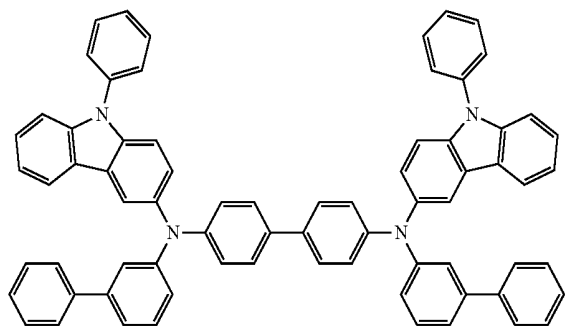
HT19
