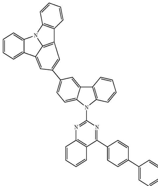
Compound 8
