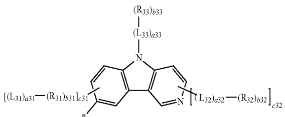
Formula 2F(2)
