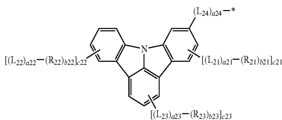
Formula 2A(3)
