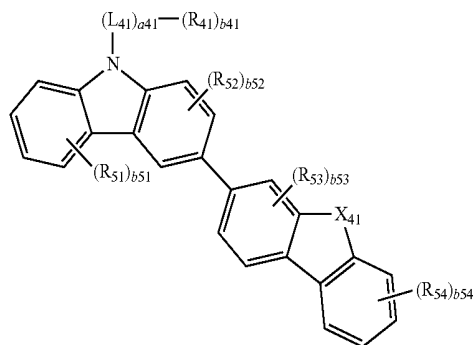
Formula 41-3
