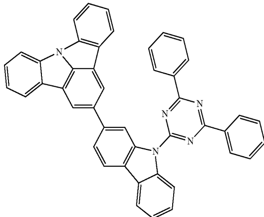
Compound 76
