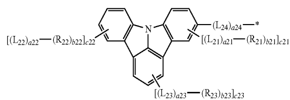
Formula 2A(4)
