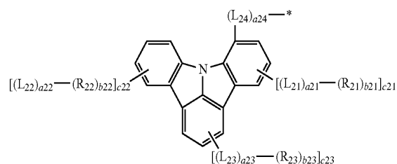
Formula 2A(2)
