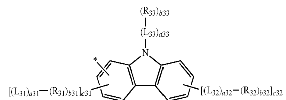
Formula 2D
