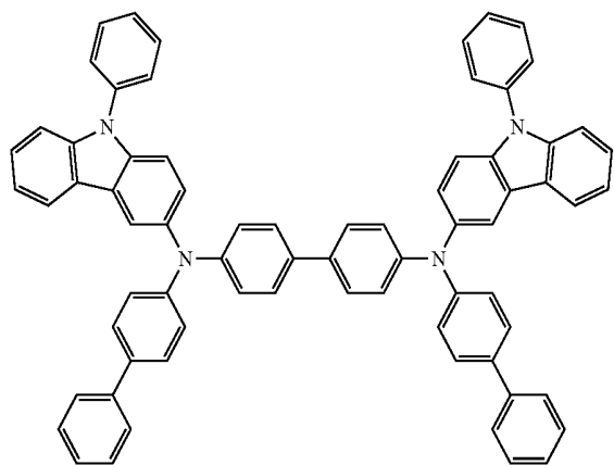
HT19
