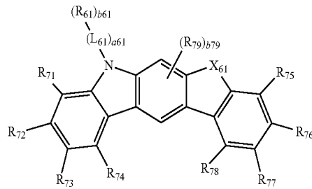
Formula 61-4
