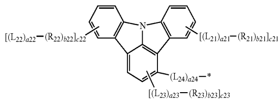
Formula 2B(2)
