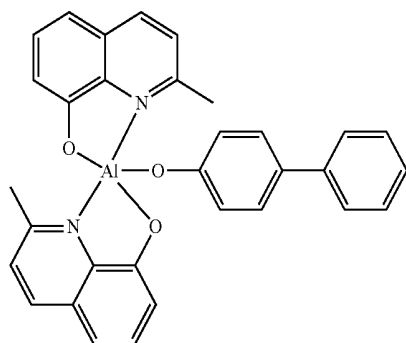
BAIq
