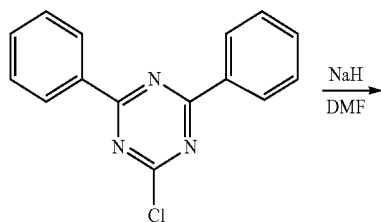
Intermediate D
