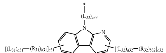
Formula 2E(4)
