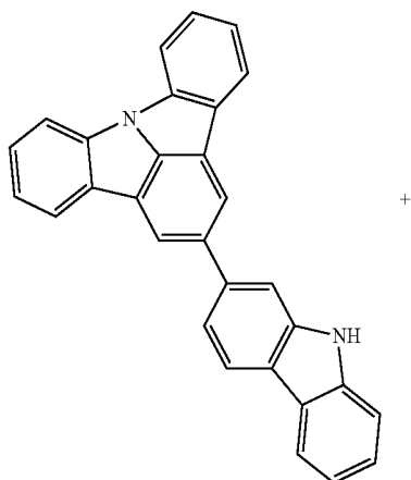
Intermediate 76-1
