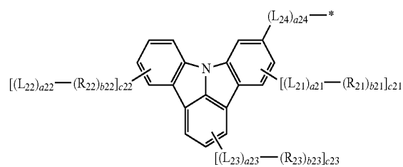
Formula 2A(3)
