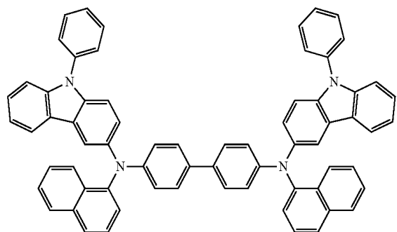
HT18
