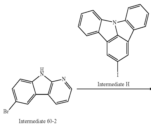
Intermediate 60-2
